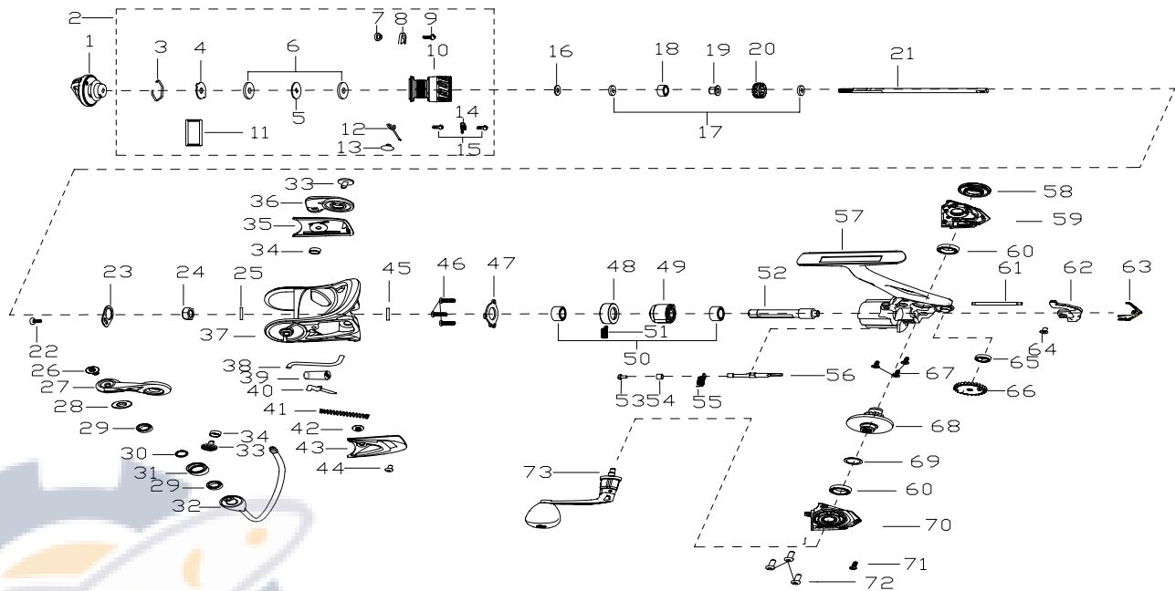
PARTS LIST OF CS6-1000
